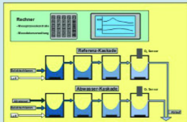
BSB – BioMonitor® analyser – functional diagram. Reproduced with kind permission of LAR AG, Berlin
