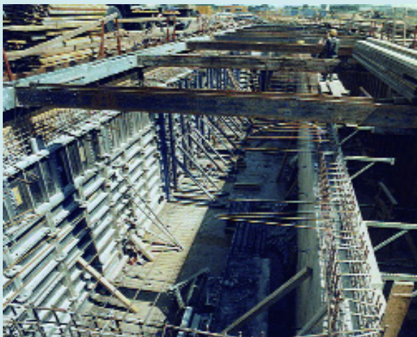
Stormwater treatment tank under construction. Reproduced with kind permission of Müller-Kalchreuth Planungsgesellschaft für Wasserwirtschaft mbH, Berlin
