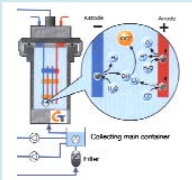
Electrochemical hypochlorite production system.
