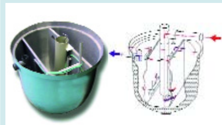
Small-scale wastewater treatment system Miniclar for 5 – 15 inhabitants.
